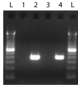
1- WT mouse DNA 2- Control plasmid DNA (pEMS1361) 3- No Template 4- Knock-in ESC line L- 100 bp ladder expected band size = 393 bp
